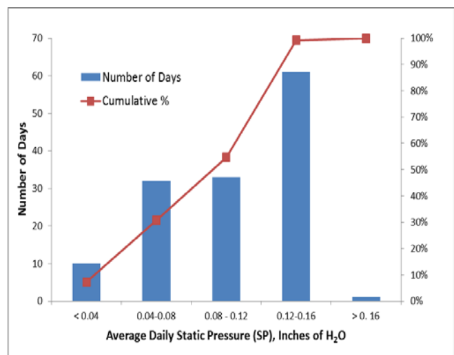
Figure 2. Distribution of average daily static pressure as measured from May to September 2012.
