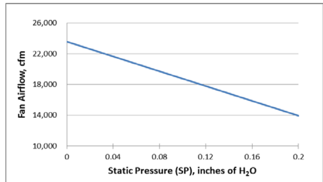
Figure 1. Average air flow vs. building static pressure, as measured in-situ from eight 52", 1.5-HP ventilation fans.
