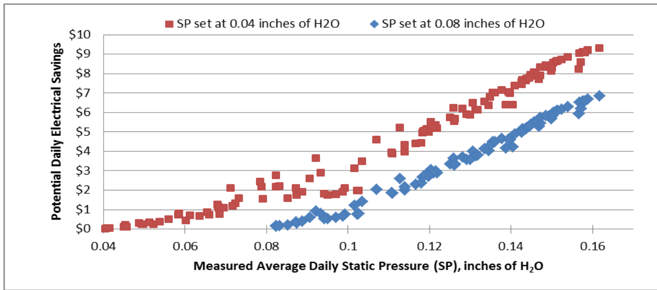
Figure 3. Potential electrical savings from May to September 2012 based on measured building ventilation rates and static pressure, relative to a baseline of 0.04" or 0.08" W.C. building static pressure.
